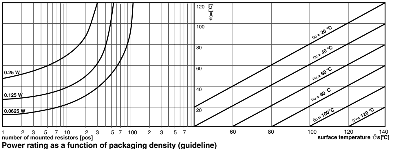
Power rating as a function of packaging density (guideline)
