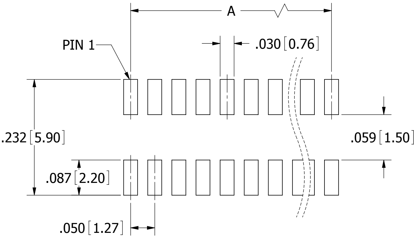
RECOMMENDED PCB SMD LAYOUT
