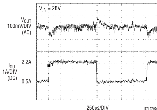
Load Step Response at V_{IN} = 28\text{V}
