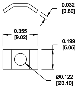
SADDLE WASHER
