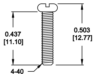
HOUSING SCREW
