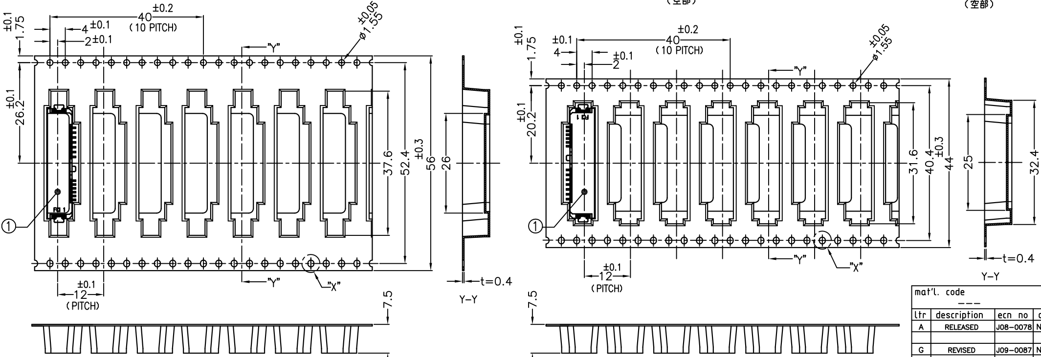
VIEW A (FREE) APPLIED TO 10085305-xxxxPELF ONLY
