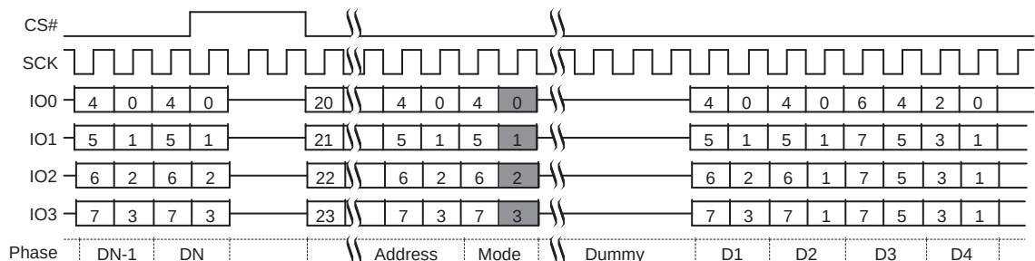
Figure 10.34 Continuous Quad I/O Read Command Sequence (3-Byte Address)
