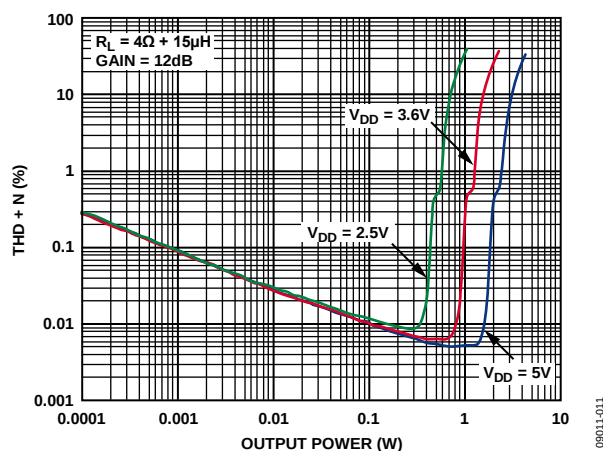
Figure 7. THD + N vs. Output Power into 4 Ω, Gain = 12 dB
