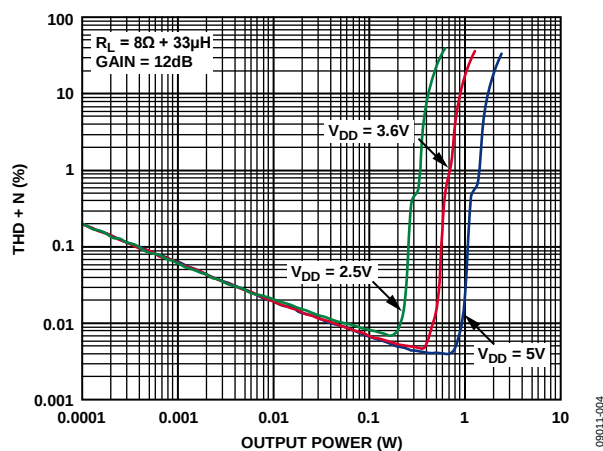
Figure 6. THD + N vs. Output Power into 8 Ω, Gain = 12 dB
