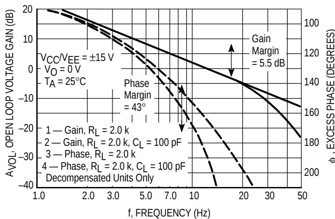
Figure 16. Open Loop Voltage Gain and Phase versus Frequency
