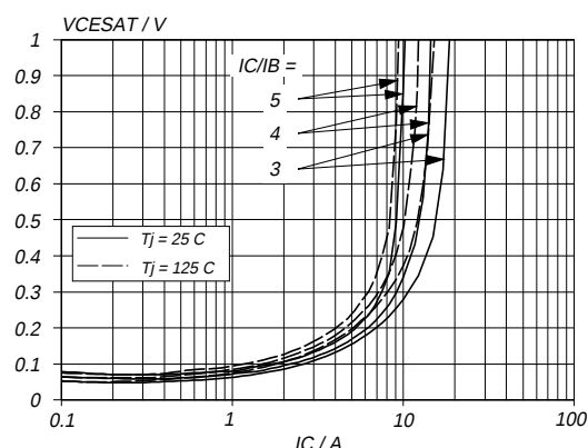
Fig. 7. Typical collector-emitter saturation voltage. V_{CEsat} = f(I_C) ; parameter I_C/I_B
