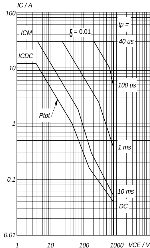
Fig.14. Forward bias safe operating area. T_{hs} = 25^\circ\text{C} I_{CDC} \& I_{CM} = f(V_{CE}) ; I_{CM} single pulse; parameter t_p Second-breakdown limits independent of temperature. Mounted with heatsink compound.
