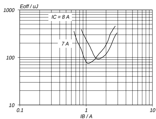
Fig. 10. Typical turn-off losses. T_j = 85^\circ\text{C} E_{off} = f(I_B) ; parameter I_C ; f = 32\text{ kHz}
