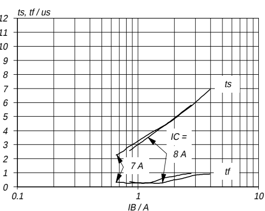
Fig. 11. Typical collector storage and fall time. t_s = f(I_B) ; t_f = f(I_B) ; parameter I_C ; T_j = 85^\circ\text{C} ; f = 32\text{ kHz}
