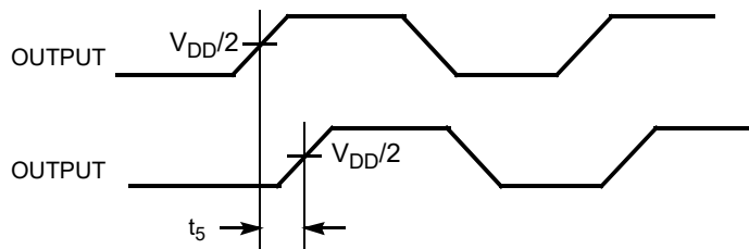
Figure 6. Input to Output Propagation Delay
