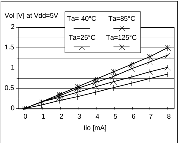
Figure 88. Typical V_{OL} at V_{DD}=5\text{V} ( \overline{\text{RESET}} )
