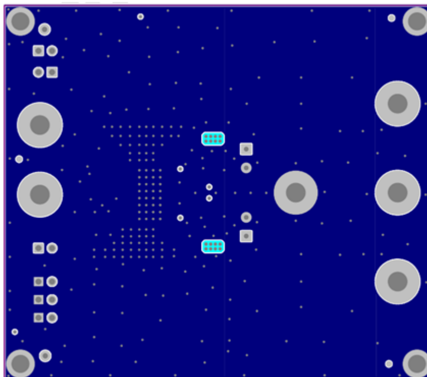
Figure 4. Bottom Composite
