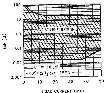
FIGURE 3. 10 \mu F ESR Range
