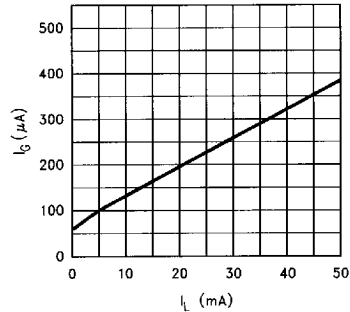
Ground Pin Current vs Load Current
