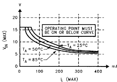
Safe Operation Boundary Curves
