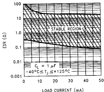
FIGURE 1. 1 \mu F ESR Range
