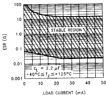
FIGURE 2. 2.2 \mu F ESR Range
