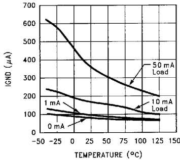
Ground Pin Current vs Temperature
