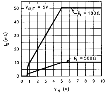
Input Current vs V_{IN}
