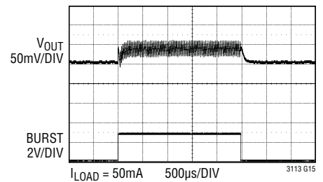
Burst to PWM Mode Transient
