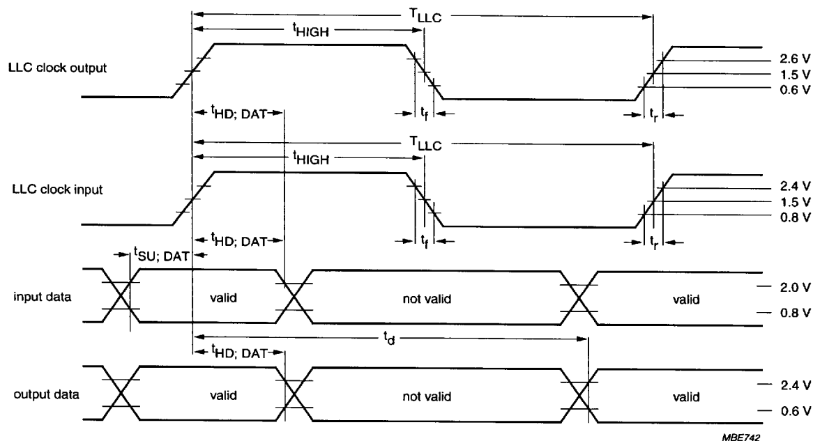
Fig.7 Clock data timing.
