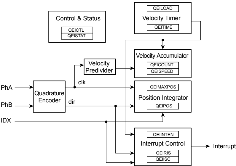
Figure 18-1. QEI Block Diagram
