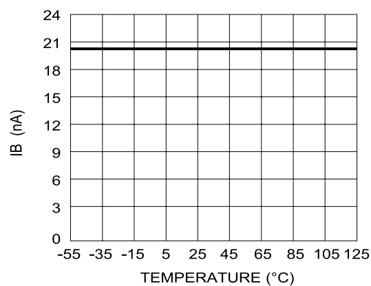
Figure 3: Input bias current vs. T_{amb}
