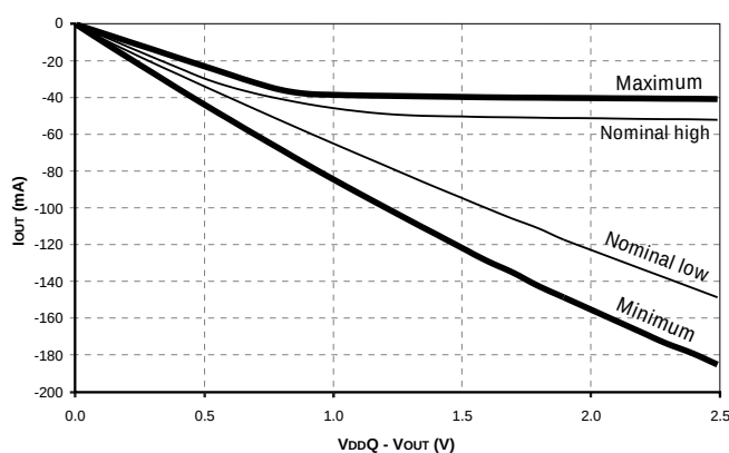
Figure 8: Pull-Up Characteristics
