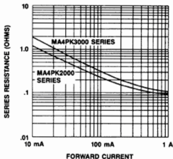
SERIES RESISTANCE vs CURRENT FREQUENCY AT 100 MHz
