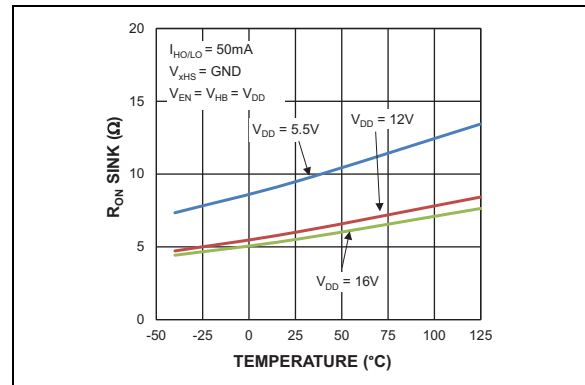
FIGURE 2-12: HO/LO Sink On-Resistance vs. Temperature.
