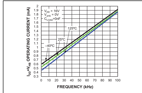
FIGURE 2-10: V_{DD+HB} Operating Current vs. Switching Frequency.
