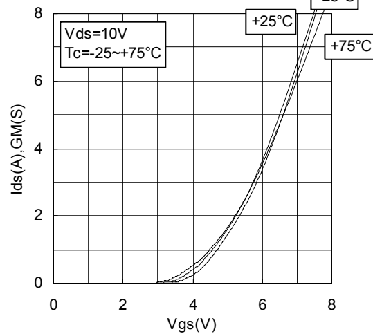
Vgs-Ids CHARACTERISTICS 2
