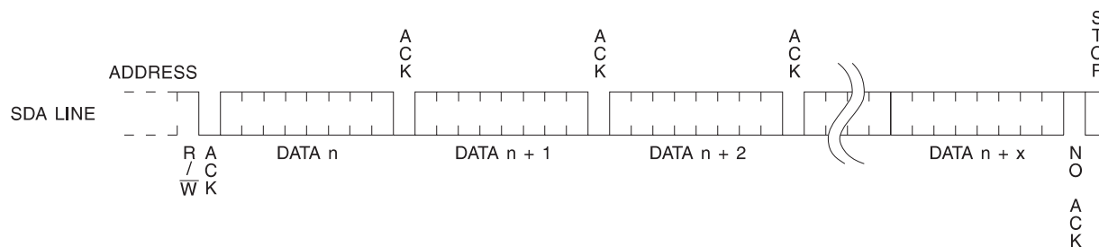
Figure 4. Sequential Read
