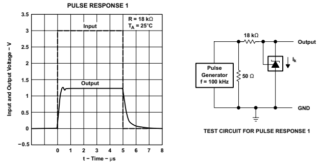
Figure 5-12. Pulse Response 1
