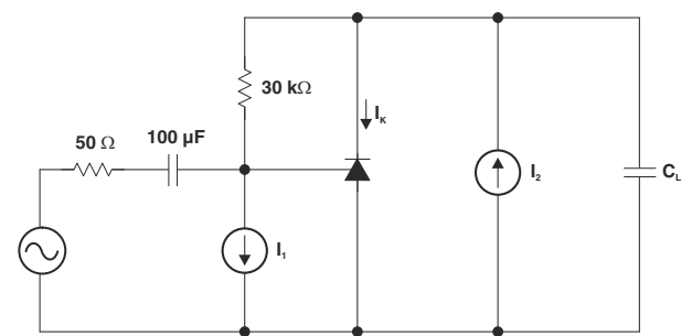
Figure 5-14. Phase Margin Test Circuit
