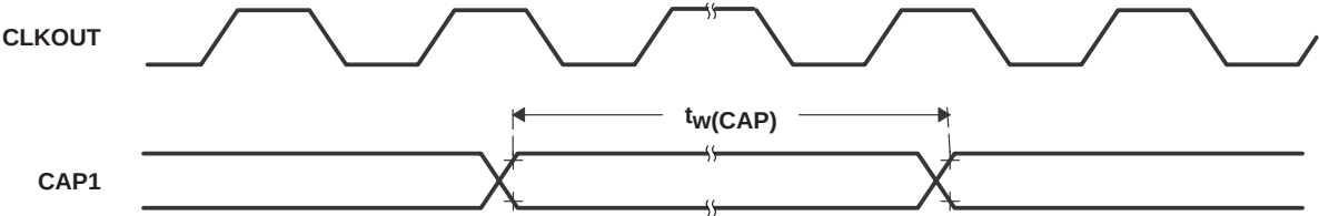
Figure 34. Capture Input Timing
