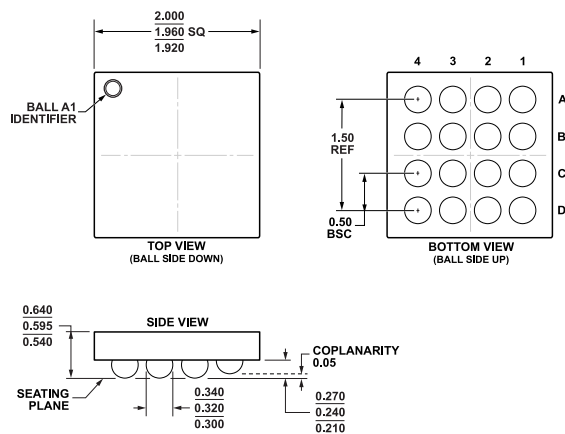
Figure 55. 16-Ball Wafer Level Chip Scale Package [WLCSP] (CB-16-3)
