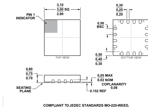
Figure 54. 16-Lead Lead Frame Chip Scale Package [LFCSP] 3 mm x 3 mm Body, Very Very Thin Quad (CP-16-32)
