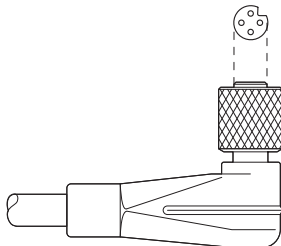
Layout of connector pin assignments
