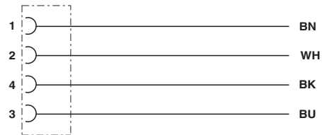
Contact assignment of the M5 socket
