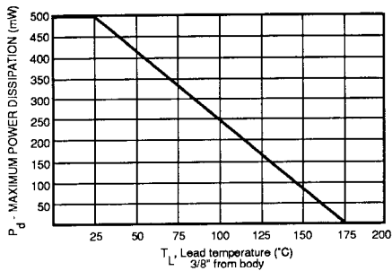
FIGURE 2 POWER-TEMPERATURE DERATING CURVE
