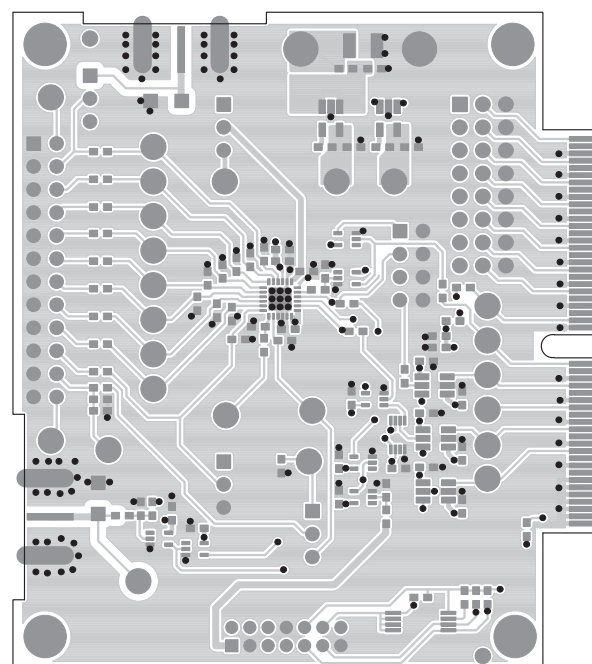
Figure 7b. Layer 1 Component Side
