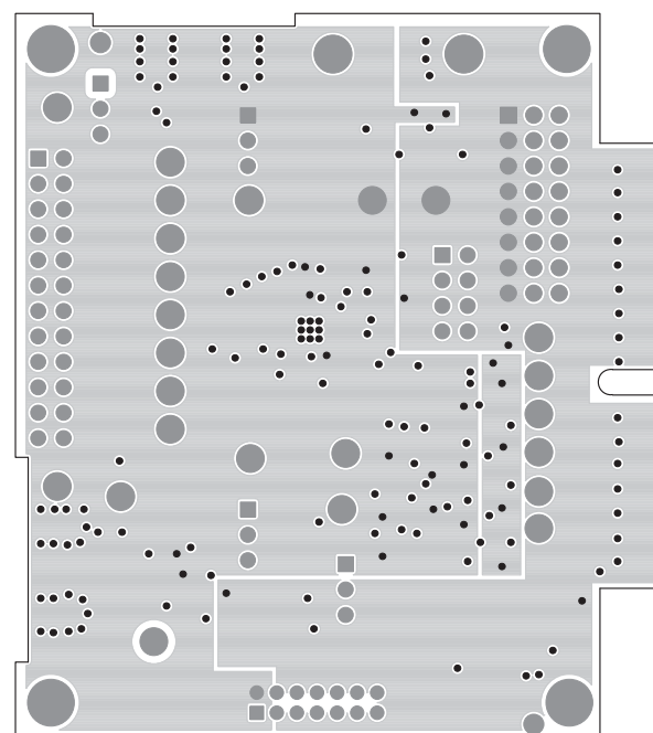
Figure 7d. Layer 3 Power Plane
