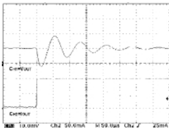
Figure 19 : Load Transient
