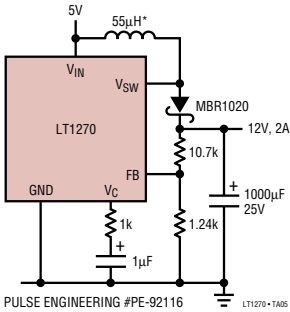
Boost Converter (5V to 12V)
