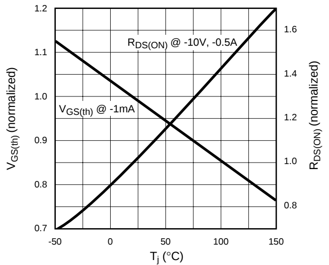
V GS(th) and R DS(ON) Variation with Temperature
