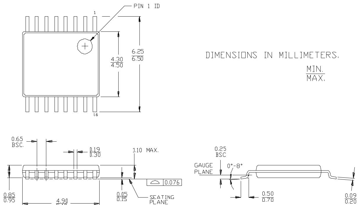
16-Lead Thin Shrink Small Outline Package (4.40 MM Body) Z16
