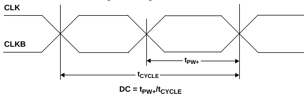
Figure 9. Duty CycleJitter
