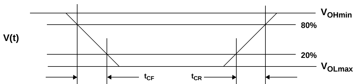
Figure 8. Voltage Waveforms
