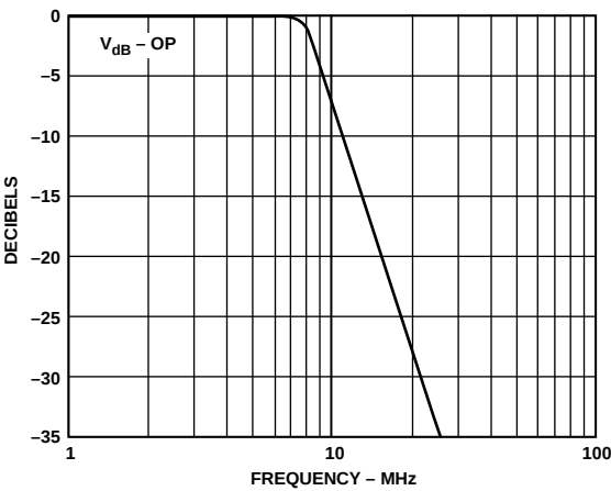
Figure 81. Output Filter Plot Close-Up
