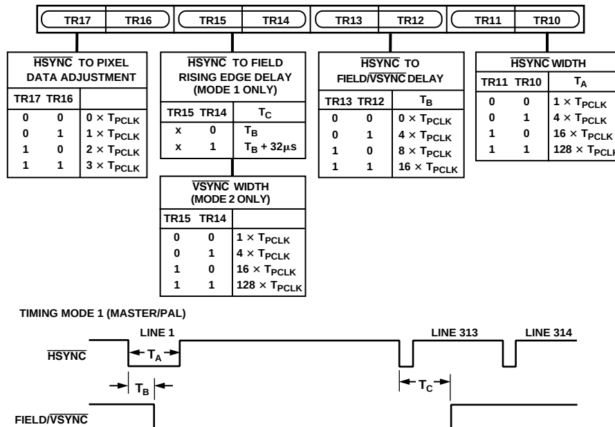
Figure 44. Timing Register 1
