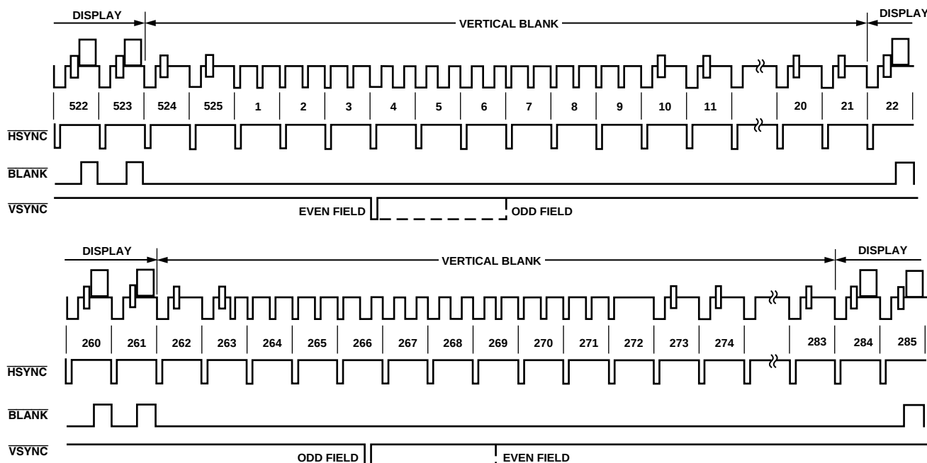
Figure 27. Timing Mode 2 (NTSC)
