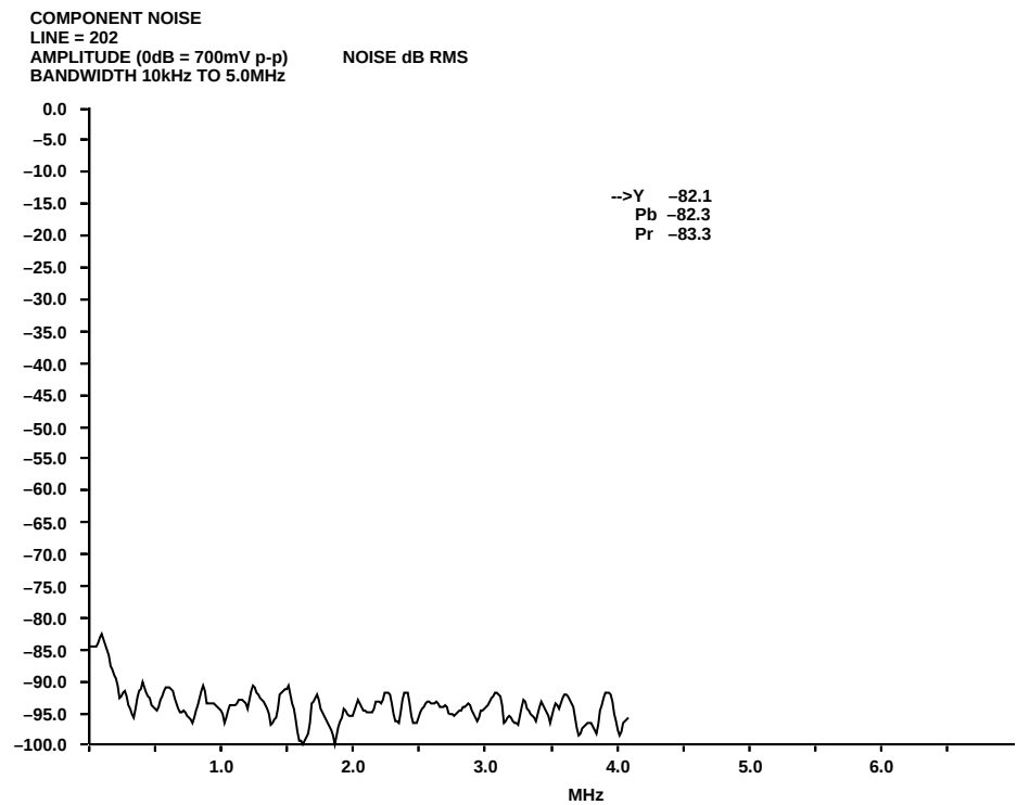
Figure 101. PAL YUV SNR Plot
