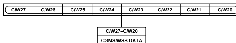
Figure 53. CGMS_WSS Register 2
