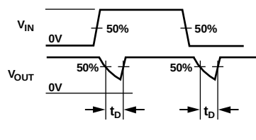
Figure 18. Break-Before-Make Time Delay, t_D
