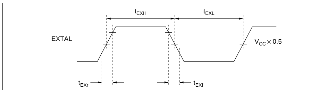
Figure 17-6 External Clock Input Timing
