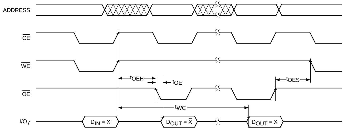
Figure 7. \overline{\text{DATA}} Polling
