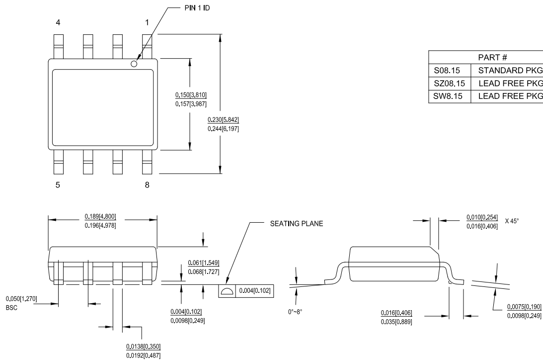
Figure 36. 8-pin SOIC (150 mils) Package Outline, 51-85066
