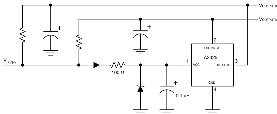
Unregulated supply
