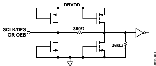
Figure 72. Equivalent SCLK/DFS or OEB Input Circuit
