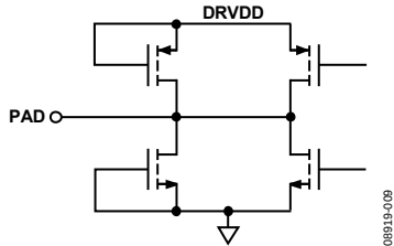
Figure 70. Digital Output
