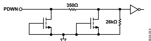
Figure 76. Equivalent PDWN Input Circuit
