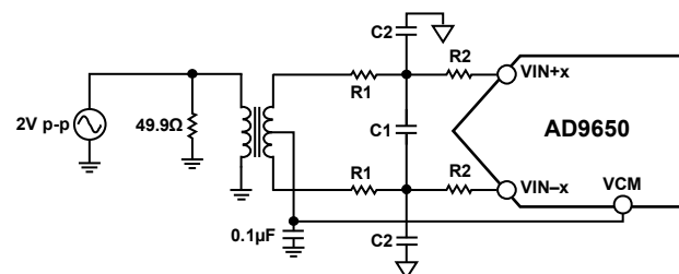
Figure 80. Differential Transformer-Coupled Configuration
