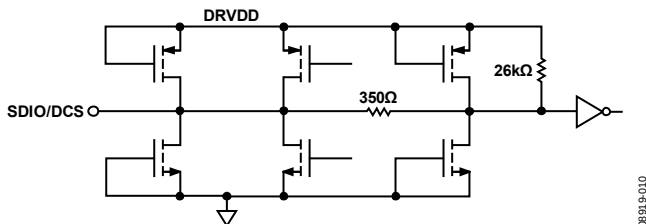
Figure 71. Equivalent SDIO/DCS Circuit
