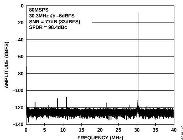
Figure 40. AD9650-80 Single-Tone FFT with f_{IN} = 30.3 MHz at -6 dBFS with Dither Enabled
