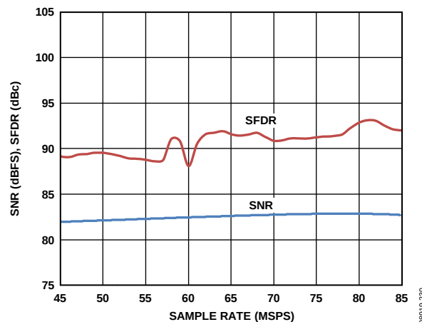
Figure 30. AD9650-65 Single-Tone SNR/SFDR vs. Sample Rate ( f_s ) with f_{IN} = 30 MHz
