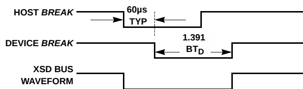
FIGURE 4A. WHEN THE HOST POWER-ON BREAK IS WIDER THAN 60µs
