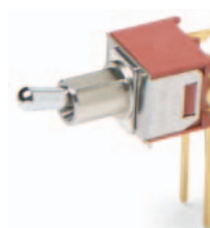
T201MH9AVBE Vertical Actuation DPDT
