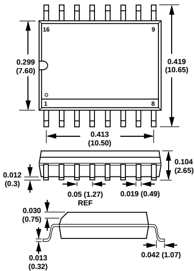
Plastic SOIC (R) Package
