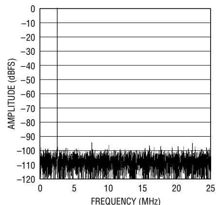
Nonaveraged, 8192 Point FFT, Input Frequency = 2.5MHz, -1dB 2V Range
