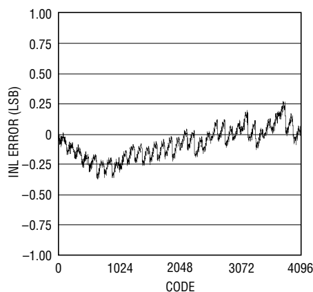
Typical INL
