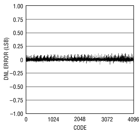
Typical DNL
