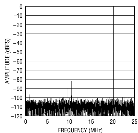
Nonaveraged, 8192 Point FFT, Input Frequency = 20MHz, -1dB 3.2V Range
