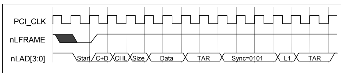
FIGURE 16 – DMA READ (FIRST BYTE)
