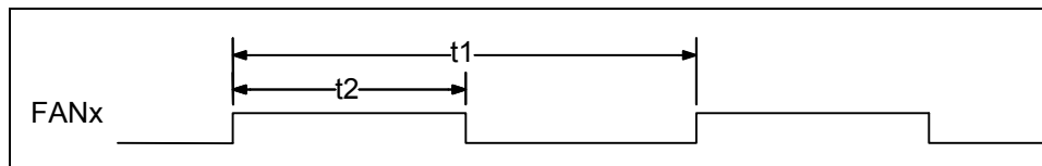
FIGURE 35 – FAN OUTPUT TIMING
