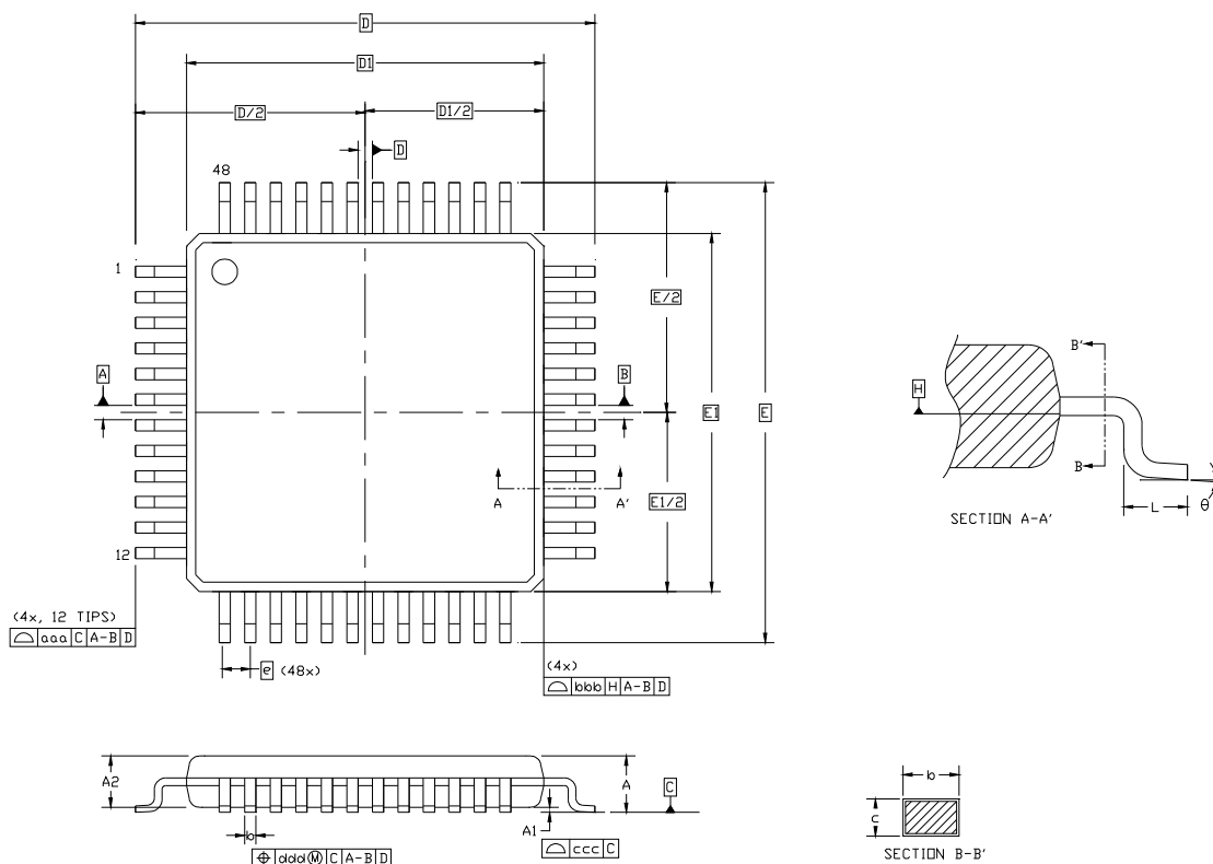
Figure 4.2. TQFP-48 Package Diagram
