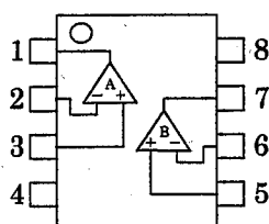
NJM12904D/12904M NJM12904E/12904V/12904R NJM12904x(PRELIMINARY)
