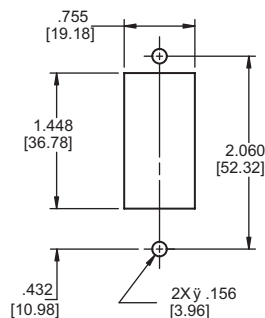
Mounting Detail
