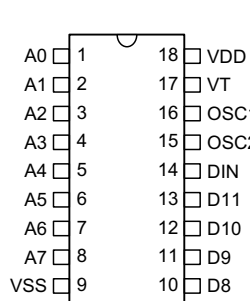
HT12D -18 DIP
