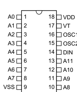
HT12F -18 DIP
