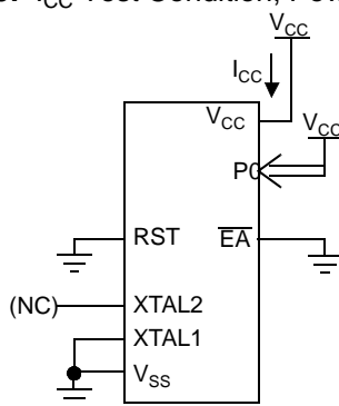
Figure 49. I_{CC} Test Condition, Power-down Mode
