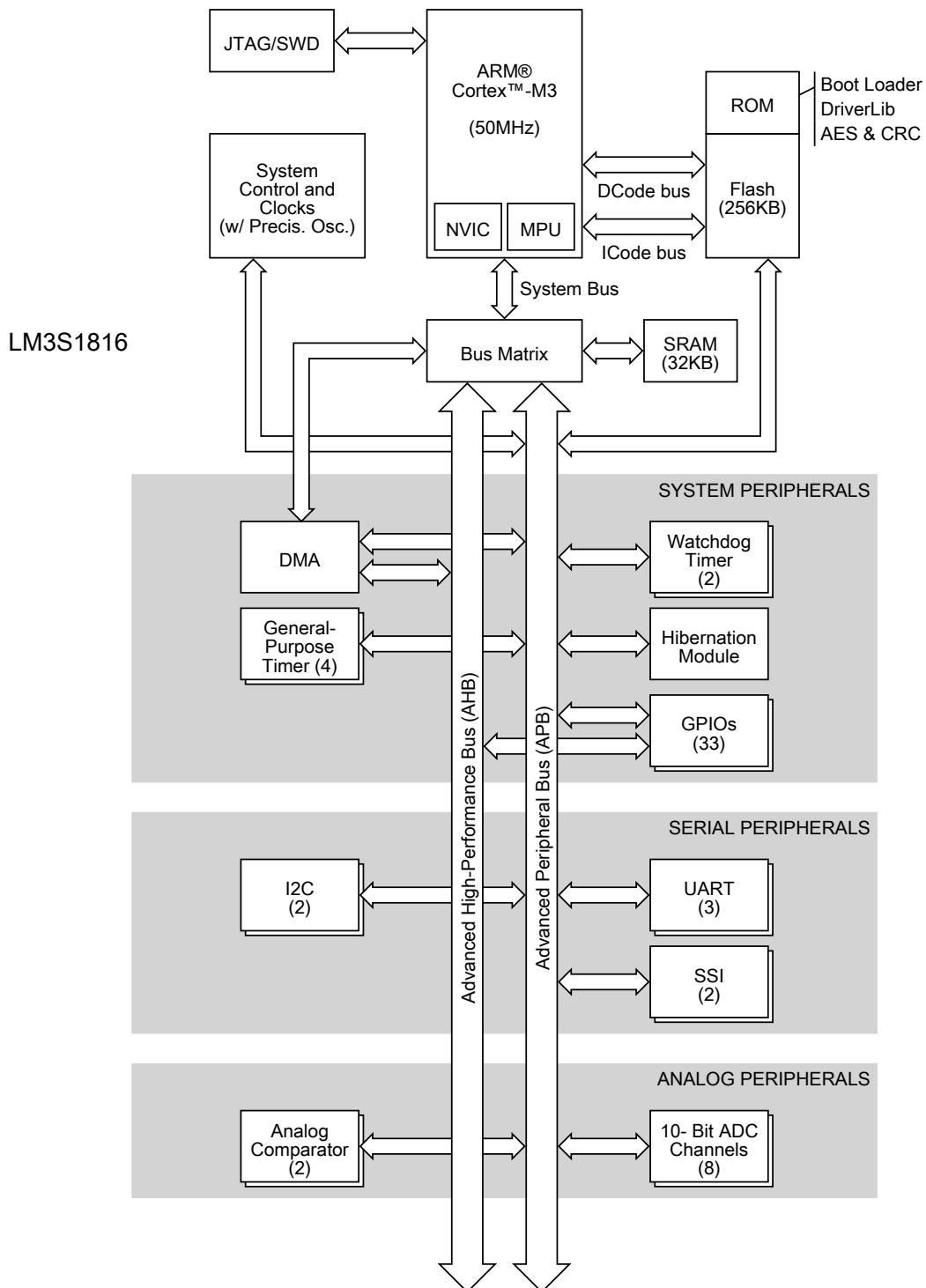
Figure 1-1. Stellaris LM3S1816 Microcontroller High-Level Block Diagram
